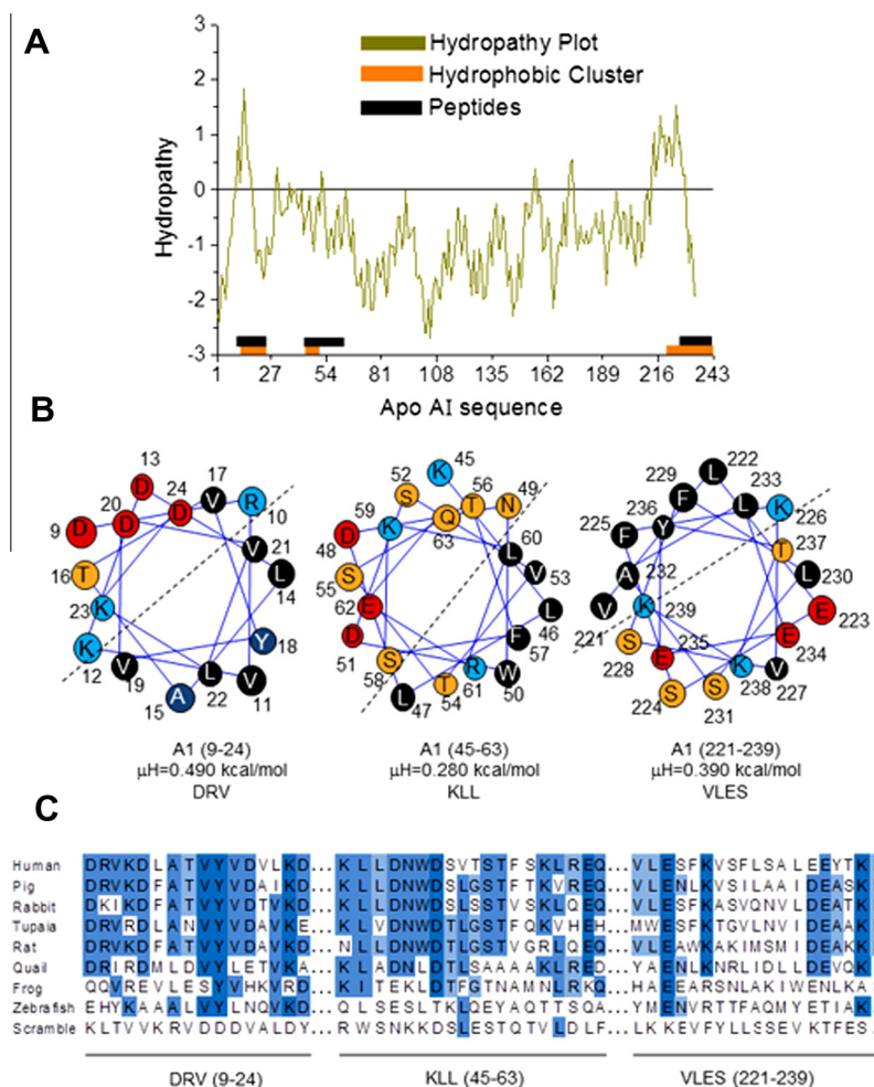
Fig. 1. Physicochemical analyses of Apo AI and Apo AI-derived peptides DRV, KLL, and VLES. (A) Hydropathy profile and hydrophobic clusters obtained in EMBOSS (orange boxes). (B) Helical wheel representation of Apo AI-derived peptides with their corresponding \mu H values. The amphipathic nature of the peptides is shown with the line indicating the polar–nonpolar interface. Black: hydrophobic residues, blue: basic residues, red: acidic residues, and yellow: polar uncharged residues. (C) Alignment of the amino acid sequence of DRV, KLL, and VLES peptides with orthologs in other species. Conserved residues are indicated.
